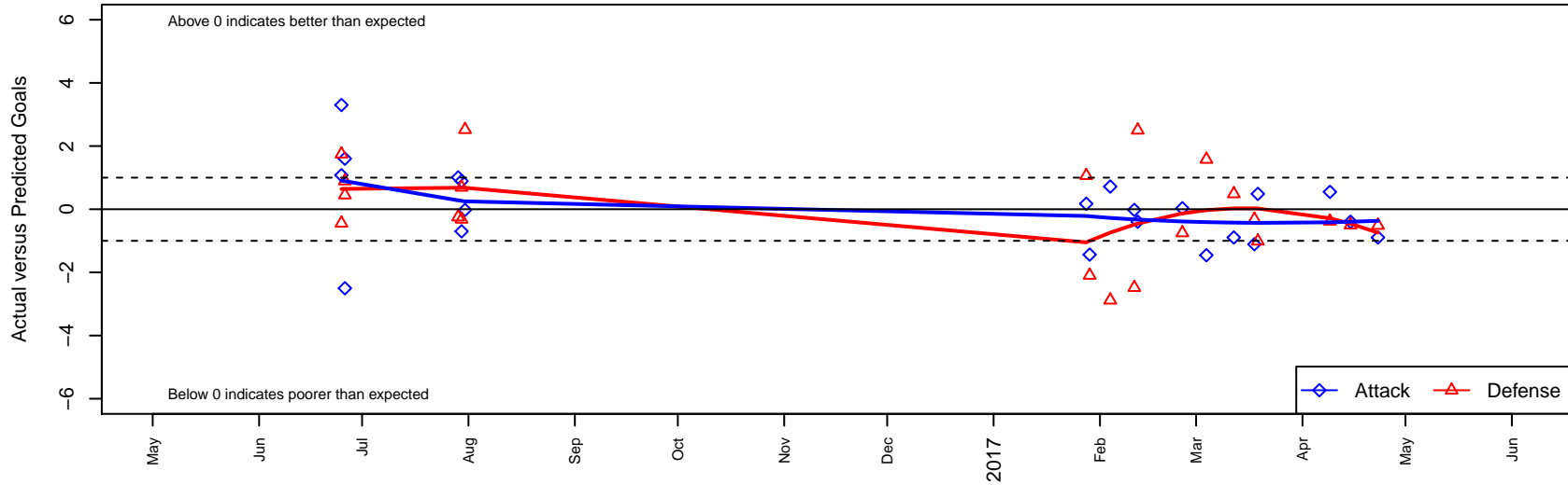
HSC River Plate B01 Dots are actual minus expected GF (blue circles) and GA (red triangles). Blue line is smoothed change in attack strength. Red is smoothed change in defense strength.
